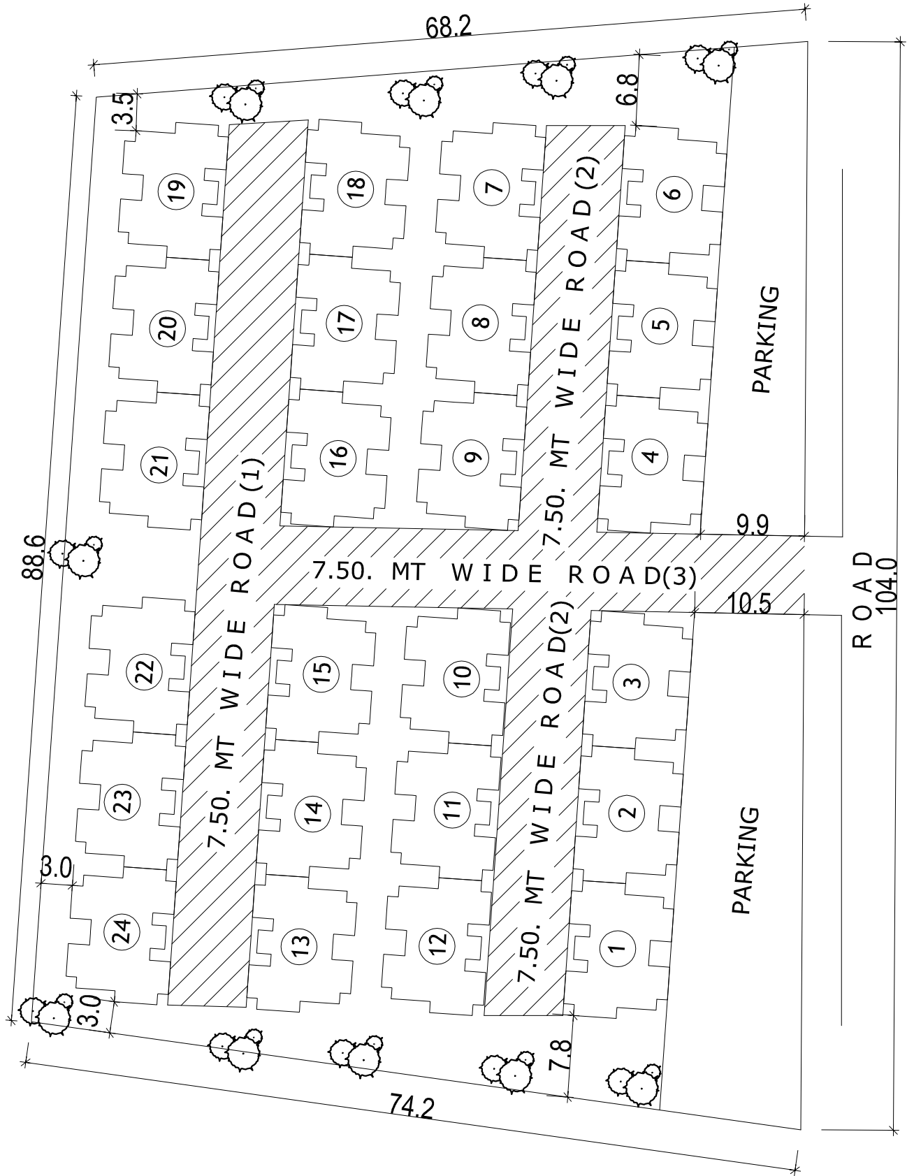
LAY-OUT OF AT T.P.NO-36,(ALTHAN) F.P. NO.-114
